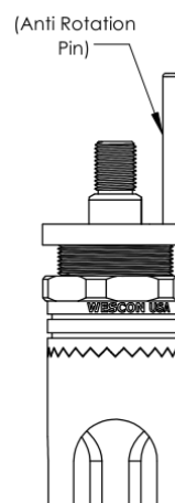
WES297-S3L-TS-AR Microstop with 1/4-28 Threaded Shank Shaft and Anti Rotation Pin
