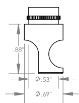
SCA Straight Cutaway Cutter Ø 1/2" (Ø 12mm)
