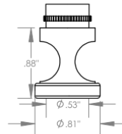
E External Thread* Cutter Ø 1/2" (Ø 12mm)
