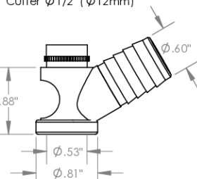
VE Vacuum External Thread Cutter \frac{1}{2} " ( \varnothing 12 mm) Choose Foot Style From Table
