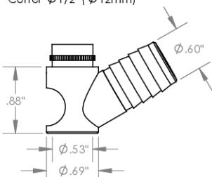
VS Vacuum Straight Cutter \frac{1}{2} " ( \varnothing 12 mm)
