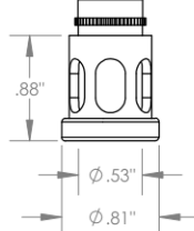
SE Slotted External Thread Cutter \frac{1}{2} " ( \varnothing 12mm) Choose Foot Style From Table
