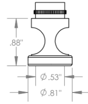
E External Thread Cutter \frac{1}{2} " ( \varnothing 12mm) Choose Foot Style From Table
