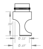
SCA Straight Cutaway Cutter \phi 1/2" ( \phi 12\text{mm} )
