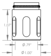
SL Slotted Cutter \phi 3/4\text{\"} (\phi 19\text{mm})
