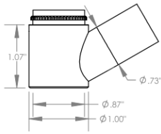
VS Vacuum Straight Cutter \phi 3/4" ( \phi 19 mm)
