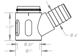
SVS Slotted Vacuum Straight Cutter \Phi 3/4" ( \Phi 19\text{mm} )
