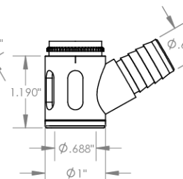
SVI Slotted Vacuum External Thread Cutter \phi 5/8" ( \phi 15\text{mm} )
