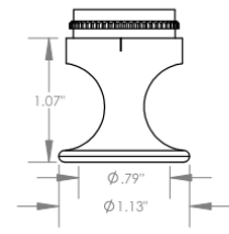
F-1125 Flanged 1.125 in OD Cutter \phi 3/4\text{\"} (\phi 19\text{mm})
