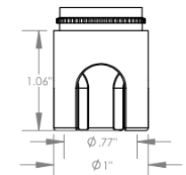
S3L 3-Leg Cutter \phi 3/4\text{\"} (\phi 19\text{mm})
