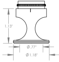
FH Flanged High Cutter \phi 3/4\text{\"} (\phi 19\text{mm})
