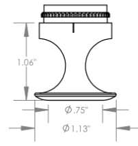
SF Spherical Flanged Cutter \phi 3/4\text{\"} (\phi 19\text{mm})
