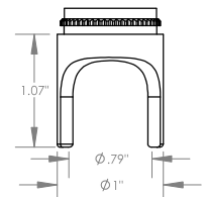
S2L 2-Leg Cutter \phi 3/4\text{\"} (\phi 19\text{mm})
