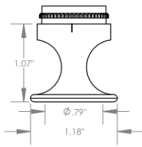
F Flanged Cutter \phi 3/4\text{\"} (\phi 19\text{mm})
