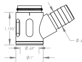
SVI Slotted Vacuum Internal Thread* Cutter \phi 5/8\text{\"} (\phi 15\text{mm})
