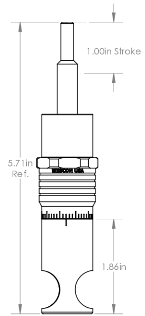
ES-1000 1.000in Shaft Travel Cutter \phi 5/8"
