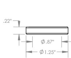
Foot Style For External Thread
