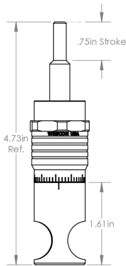
ES-750 .750in Shaft Travel Cutter \phi 5/8"
