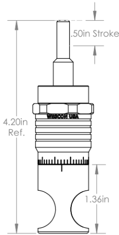
ES-500 .500in Shaft Travel Cutter \phi 5/8"
