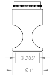
S Straight Cutter \phi 3/4" ( \phi 19\text{mm} )
