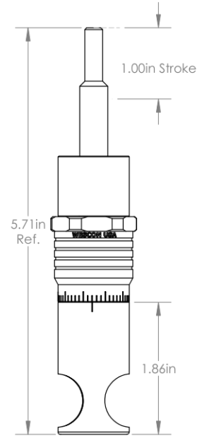
ES-1000 1.000in Shaft Travel Cutter \phi 5/8"
