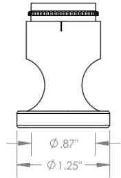
E External Thread Cutter \phi 3/4" ( \phi 19\text{mm} ) Choose Foot Style From Table
