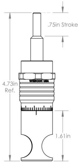
ES-750 .750in Shaft Travel Cutter \phi 5/8"
