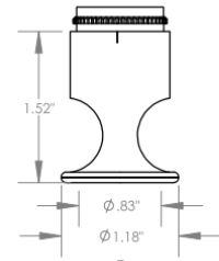
F Flanged Cutter \phi 3/4" ( \phi 19 mm)
