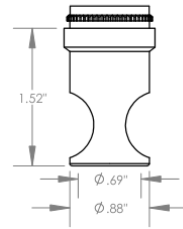
S-875 Straight 0.875in OD Cutter \phi 5/8" ( \phi 15 mm)
