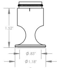
F Flanged Cutter \phi 3/4" ( \phi 19\text{mm} )
