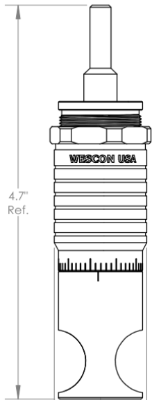
WES596-EXA-S Microstop with 1/4" Standard Shaft
