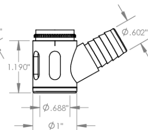
SVI Slotted Vacuum External Thread Cutter \phi 5/8" ( \phi 15\text{mm} )
