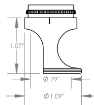
FCA Flanged Cutaway Cutter \varnothing 3/4" ( \varnothing 19\text{mm} )
