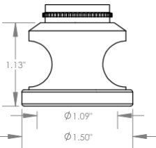
BWE Bell Wide External Thread* Cutter \varnothing 1" ( \varnothing 25\text{mm} )
