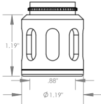
SBI Slotted Bell Internal Thread* Cutter \varnothing 3/4" ( \varnothing 19\text{mm} )
