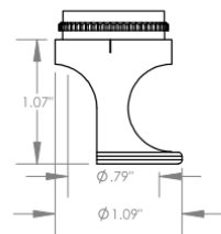
FCA Flanged Cutaway Cutter \varnothing 3/4" ( \varnothing 19\text{mm} )
