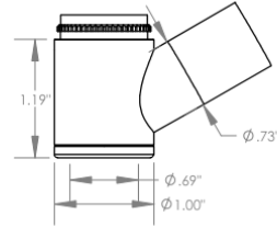
VI Vacuum Internal Thread* Cutter \frac{5}{8} " (15mm)
