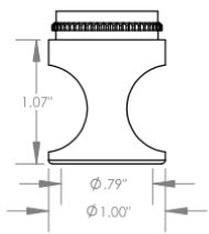
S Straight Cutter \varnothing 3/4" ( \varnothing 19\text{mm} )
