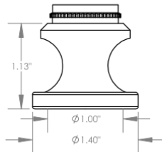
BE Bell External Thread* Cutter \varnothing 7/8" ( \varnothing 22\text{mm} )
