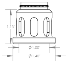
SBE Slotted Bell External Thread* Cutter \varnothing 7/8" ( \varnothing 22\text{mm} )
