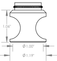
B Bell Cutter \varnothing 7/8" ( \varnothing 22\text{mm} )
