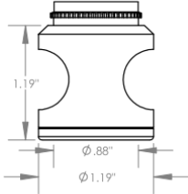
BI Bell Internal Thread* Cutter \varnothing 3/4" ( \varnothing 19\text{mm} )
