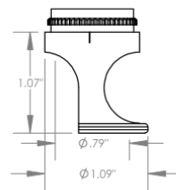
FCA Flanged Cutaway Cutter \varnothing 3/4" ( \varnothing 19\text{mm} )
