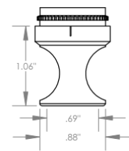
S-875 Straight 0.875 in OD Cutter \varnothing 5/8" ( \varnothing 15\text{mm} )
