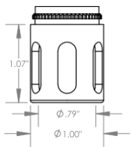
SL Slotted Cutter \varnothing 3/4" ( \varnothing 19\text{mm} )
