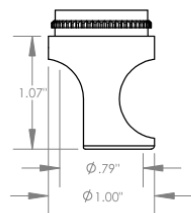
SCA Straight Cutaway Cutter \varnothing 3/4" ( \varnothing 19\text{mm} )
