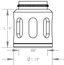
SBI Slotted Bell Internal Thread* Cutter \varnothing 3/4" ( \varnothing 19\text{mm} )
