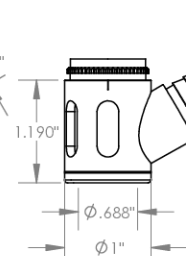
SVI Slotted Vacuum External Thread Cutter \phi 5/8 " ( \phi 15 mm)
