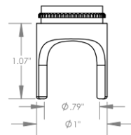
S2L 2-Leg Cutter \phi 3/4\text{\"} (\phi 19\text{mm})
