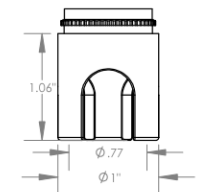
S3L 3-Leg Cutter \phi 3/4\text{\"} (\phi 19\text{mm})
