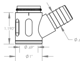
SVI Slotted Vacuum Internal Thread* Cutter \phi 5/8\text{\"} (\phi 15\text{mm})
