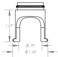
F2L Flanged 2-Leg Cutter \phi 3/4\text{\"} (\phi 19\text{mm})
