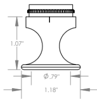
F Flanged Cutter \phi 3/4\text{\"} (\phi 19\text{mm})
