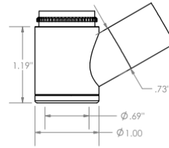
VI Vacuum Internal Thread* Cutter \frac{5}{8} " ( \varnothing 15 mm)
