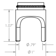
S2L 2-Leg Cutter \phi 3/4" ( \phi 19\text{mm} )
