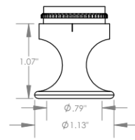
F-1125 Flanged 1.125 in OD Cutter \phi 3/4\text{\"} (\phi 19\text{mm})
