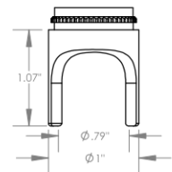
S2L 2-Leg Cutter \phi 3/4\text{\"} (\phi 19\text{mm})
