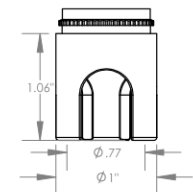
S3L 3-Leg Cutter \phi 3/4\text{\"} (\phi 19\text{mm})
