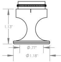
FH Flanged High Cutter \Phi 3/4" ( \Phi 19 mm)
