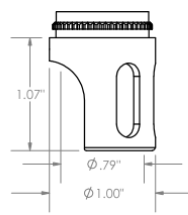
SSCA Slotted Straight Cutaway Cutter \phi 3/4" ( \phi 19\text{mm} )
