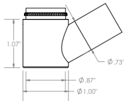
VS Vacuum Straight Cutter \frac{3}{4} " ( \varnothing 19mm)
