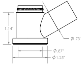
VE Vacuum External Thread* Cutter \Phi 3/4 " ( \Phi 19 mm)
