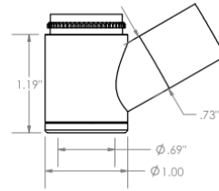
VI Vacuum Internal Thread* Cutter \Phi 5/8 " ( \Phi 15 mm)
