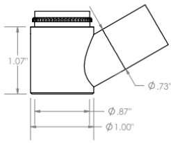
VS Vacuum Straight Cutter \Phi 3/4 " ( \Phi 19 mm)
