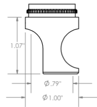
SCA Straight Cutaway Cutter \phi 3/4 " ( \phi 19 mm)
