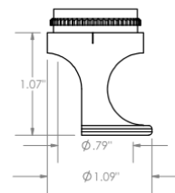
FCA Flanged Cutaway Cutter \phi 3/4 " ( \phi 19 mm)
