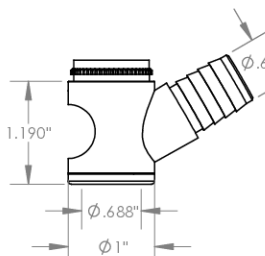
WVI Vacuum Internal Thread Cutter \phi 5/8" ( \phi 15 mm)
