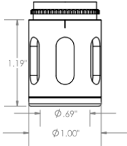
SI Slotted Internal Thread* Cutter \varnothing 5/8" ( \varnothing 15\text{mm} )
